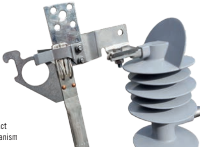
150BIL HVI with Earthing Stirrup
