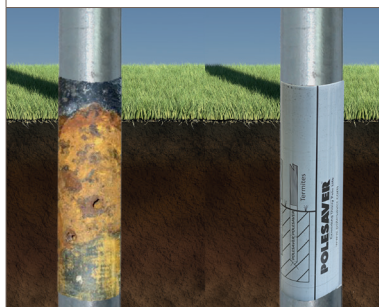
Steel Poles
