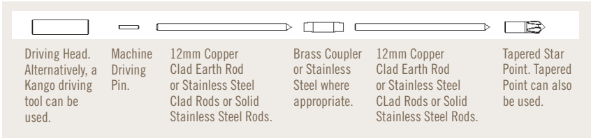
Earth Rod Configuration
