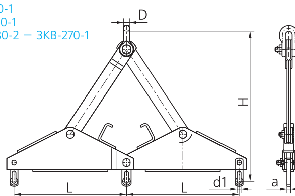
Balancing yokes of 3KB type with one attachment point are intended for insulating strings of power lines. Balancing yokes meet TU 3449-112-0011120-95 requirements.
