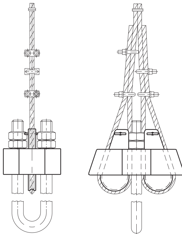
Clamp installation chart
