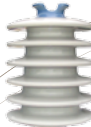
NZI 33kV ALP33/920 Tie Top Pin Type Part No. 115029 Made in NZ
